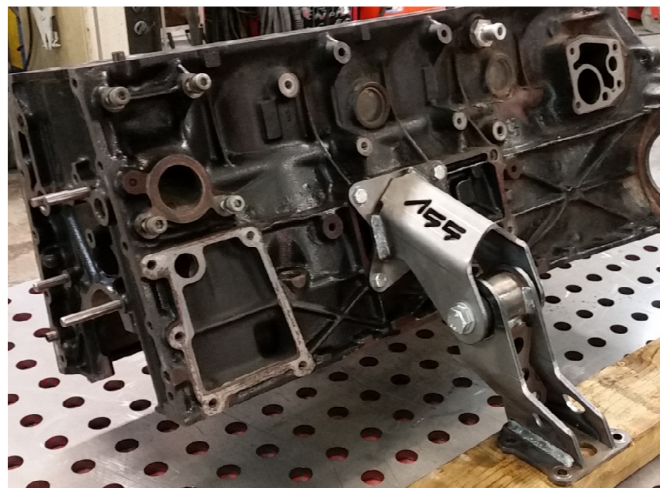
Insug-sida
